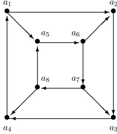
FIGURE 2. Graph G_1 of type (K)
