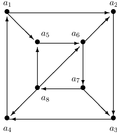
FIGURE 3. Graph G_2 of type (H)
