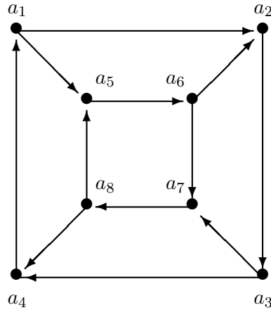
FIGURE 4. Graph G_3 of type (CK)
