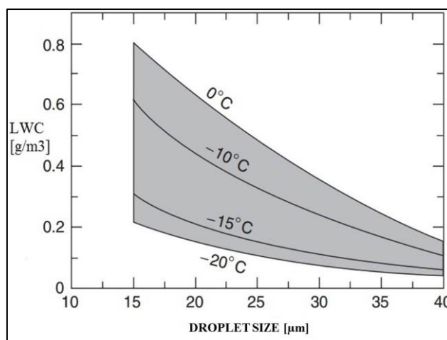
Figure 7. Icing according to temperature and liquid water content (LWC) (the grey area highlights the conditions in which the aircraft has to safely execute its flight tasks in order to get a licence to fly among icing) [24]
