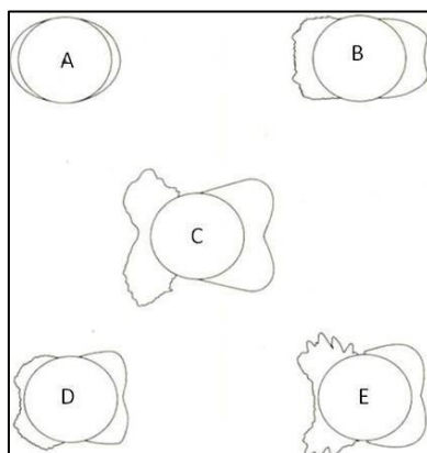
Figure 13. Certain possible forms of ice accretion [32]
