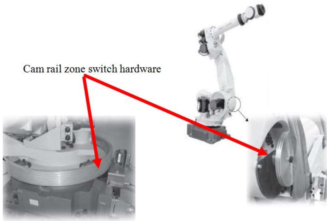
Fig. 8 shows axis 1 and 2 of a robot that are secured in a two-channelled hardware way
